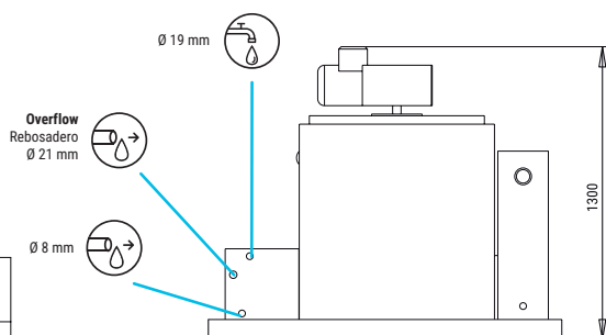
FRONTAL VIEW VISTA FRONTAL
